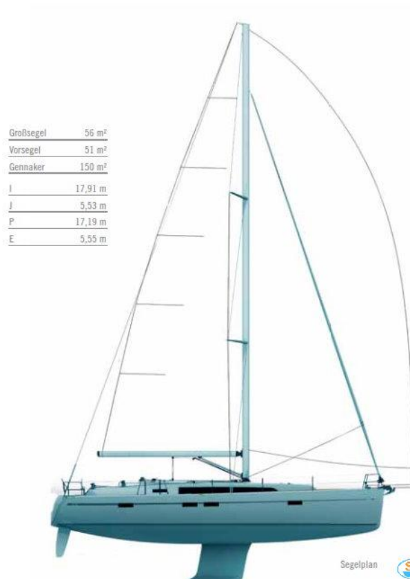
Layout / Bavaria Cruiser 46 - 2014
