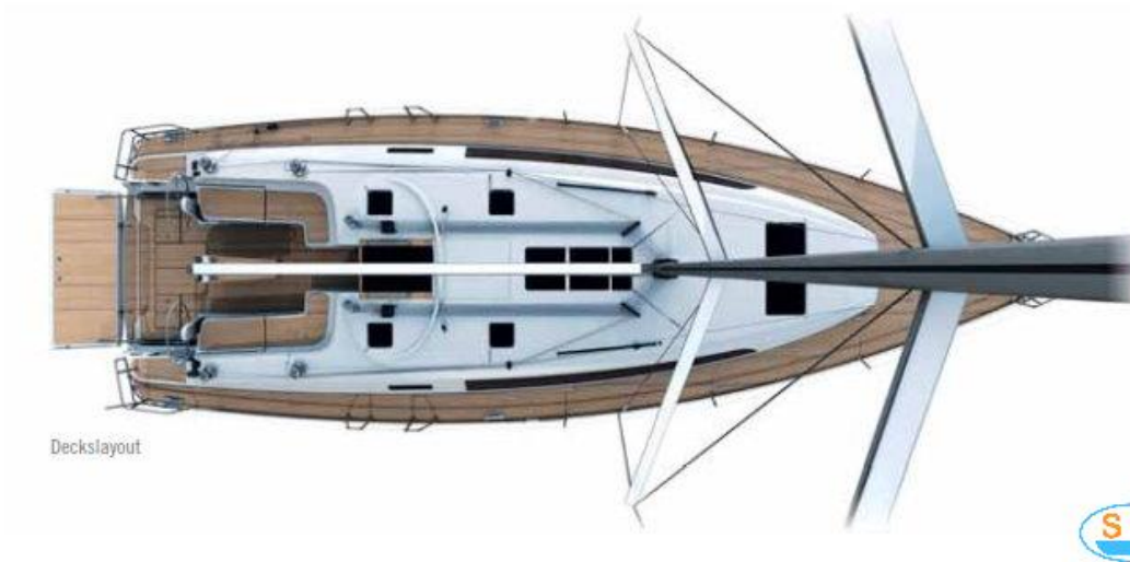
Layout / Bavaria Cruiser 46 - 2014
